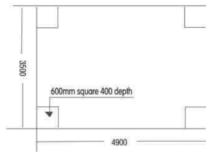
Foundation drawing
